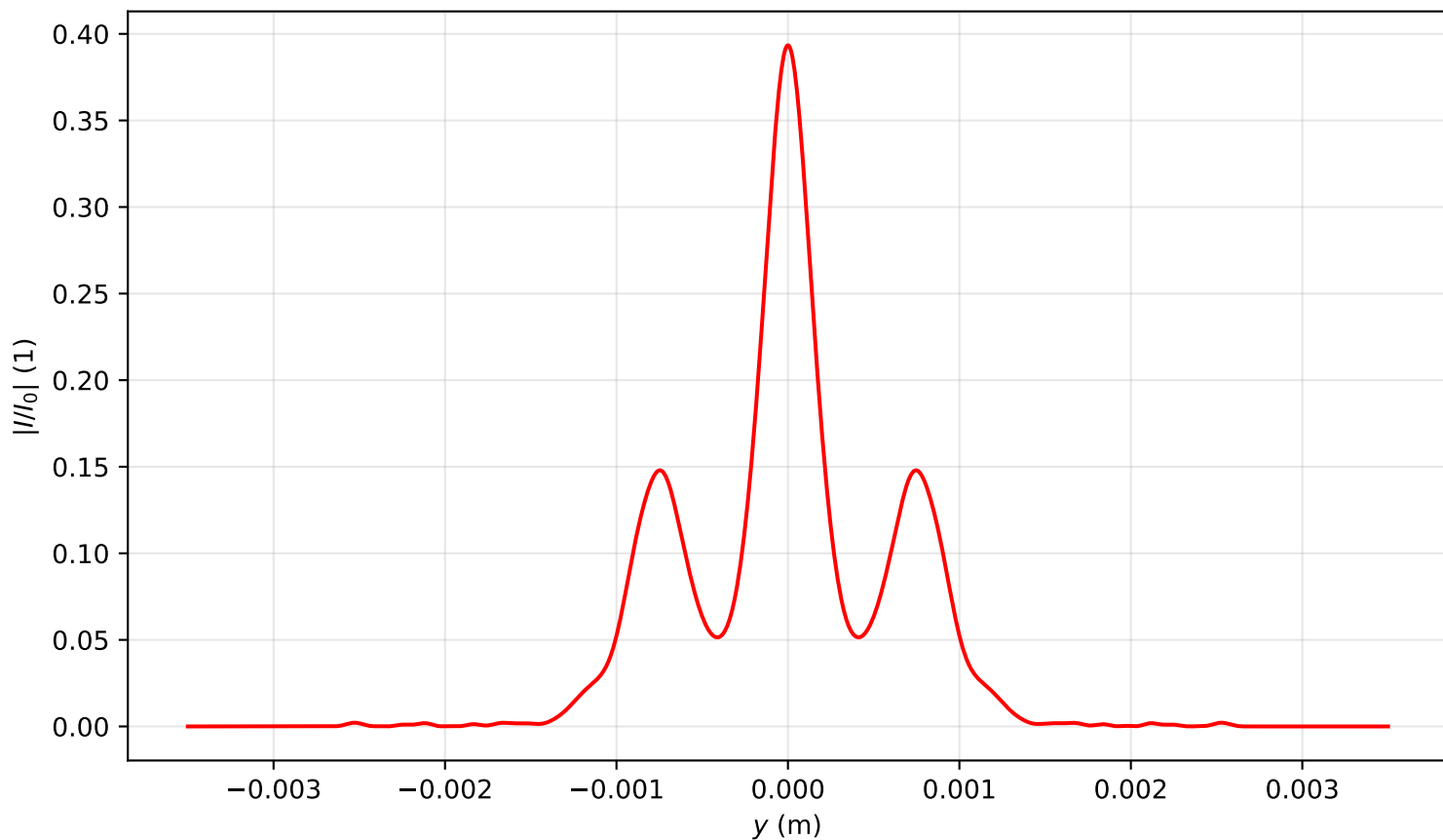
Intensity profile I(x=0, y, z=1.911)/I_0 , P_{in}=7.5P_{cr} , artificial time
